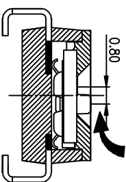
[装配行程]
